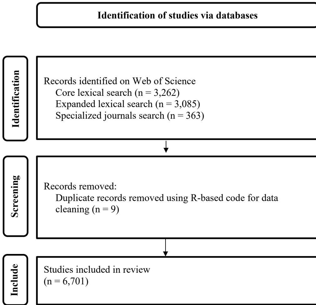
Figure 1. PRISMA chart.
